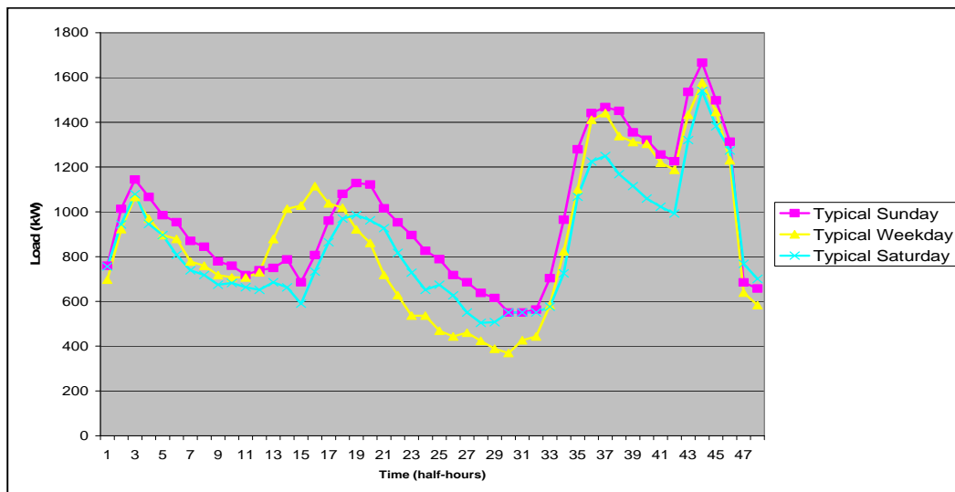
FIGURE 1: Average electricity demand for the 400 residents in the Halswell suburb during the winter month of July 2006. The last peak represents network controlled water heating loads. Time is quoted in 30 minutes intervals from midnight
